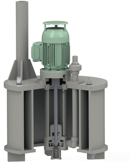
Model D0-D Float mounted sump pump
