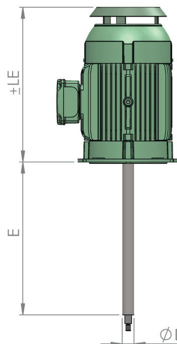
DW Motor
