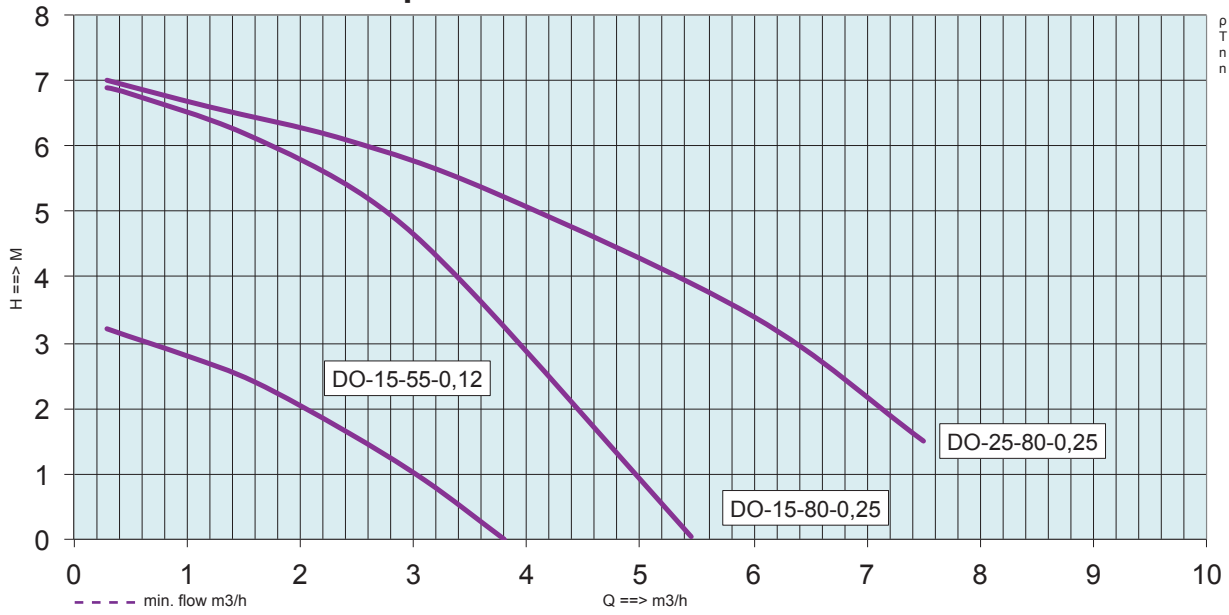
PERFORMANCE CURVES 2-pole motors 50 - 60 Hz
