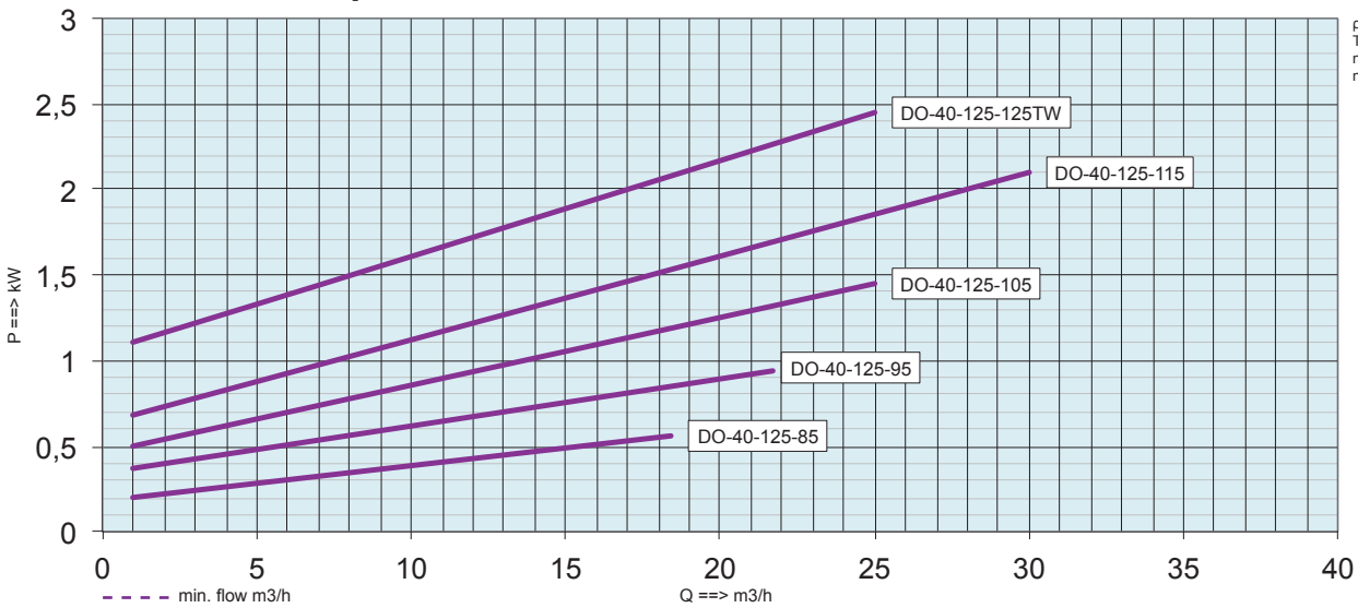
POWER CURVES 2-pole motors 50 - 60 Hz
