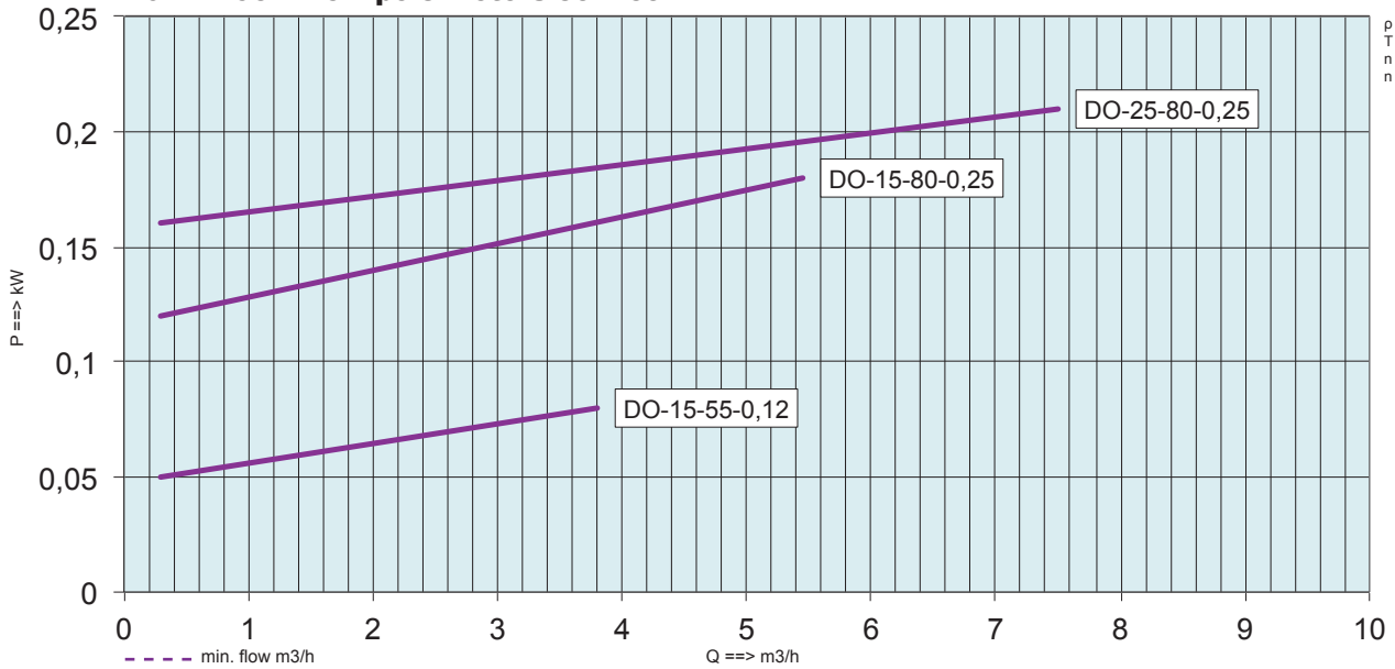
POWER CURVES 2-pole motors 50 - 60 Hz
