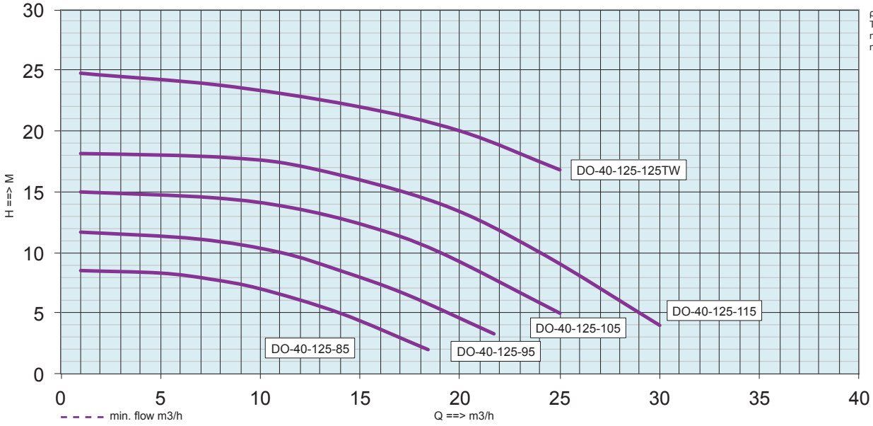
PERFORMANCE CURVES 2-pole motors 50 - 60 Hz
