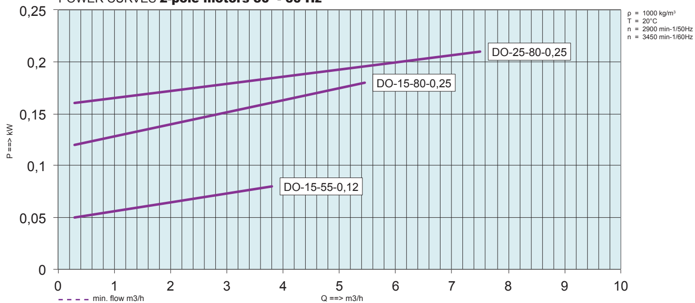
POWER CURVES 2-pole motors 50 - 60 Hz
