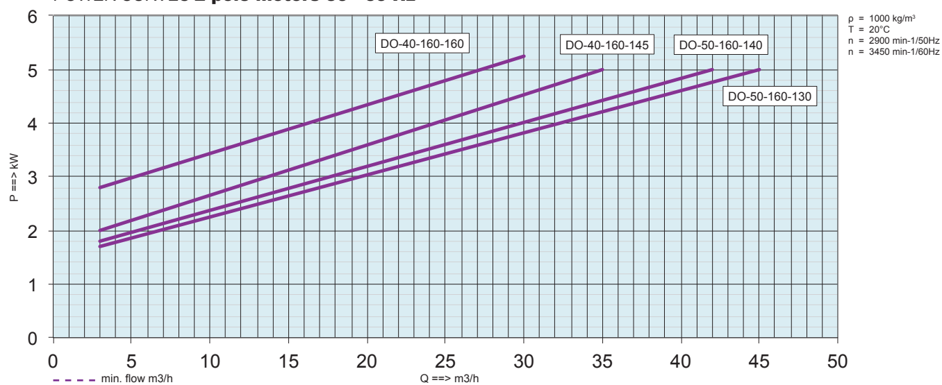
POWER CURVES 2-pole motors 50 - 60 Hz
